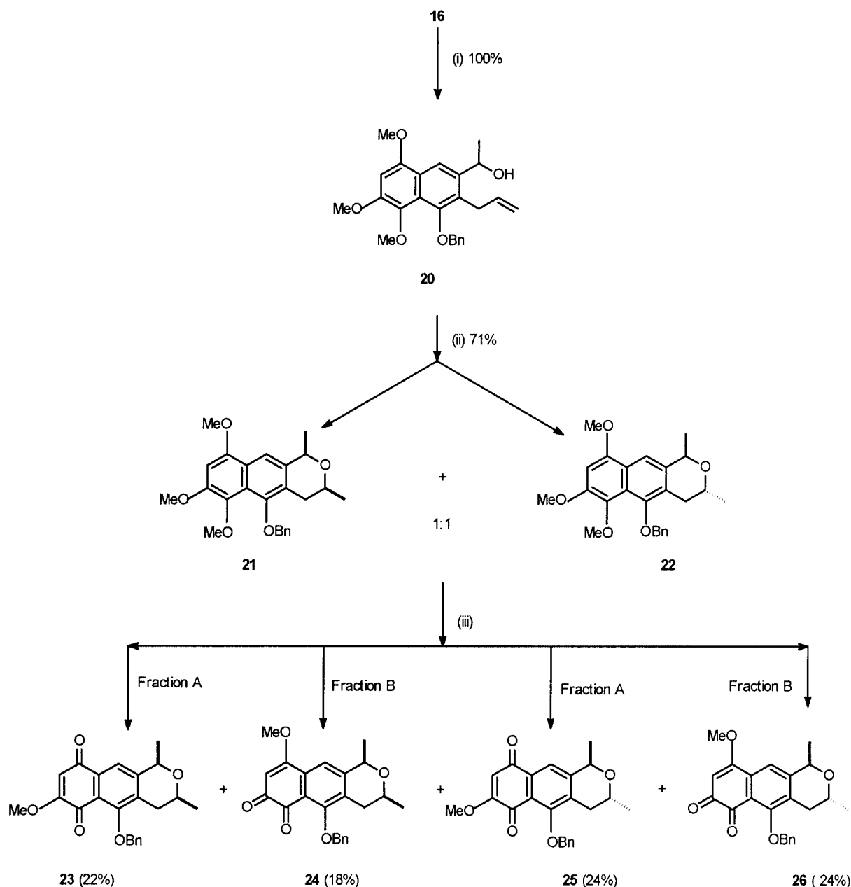
Scheme 2. Reagents and conditions: (i) MeMgBr/diethyl ether; (ii) Hg(OAc) 2 /THF/H 2 O/NaOH/NaBH 4 ; (iii) cerium(IV) ammonium nitrate/H 2 O/CH 3 CN
