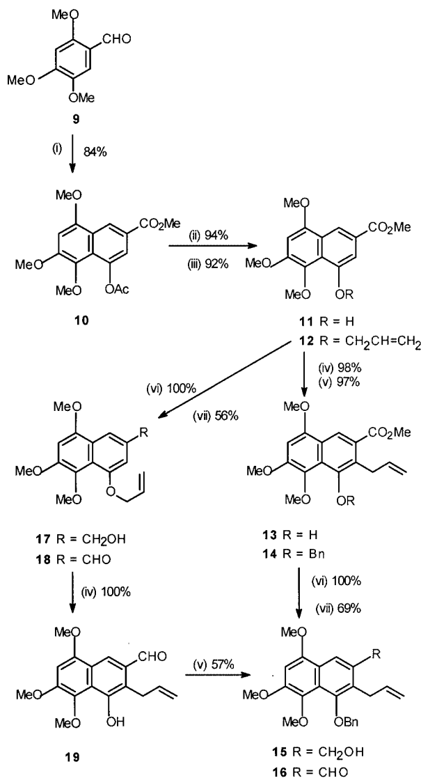
Scheme 1. Reagents and conditions: (i) dimethyl malonate/KO t Bu/ tert -butyl alcohol reflux then NaOAc/Ac 2 O reflux; (ii) 1% KOH/MeOH; (iii) allyl bromide/K 2 CO 3 /acetone/reflux; (iv) 180 °C/N 2 ; (v) BnBr/K 2 CO 3 /acetone/reflux; (vi) LAH/THF; (vii) MnO 2 /benzene/reflux
