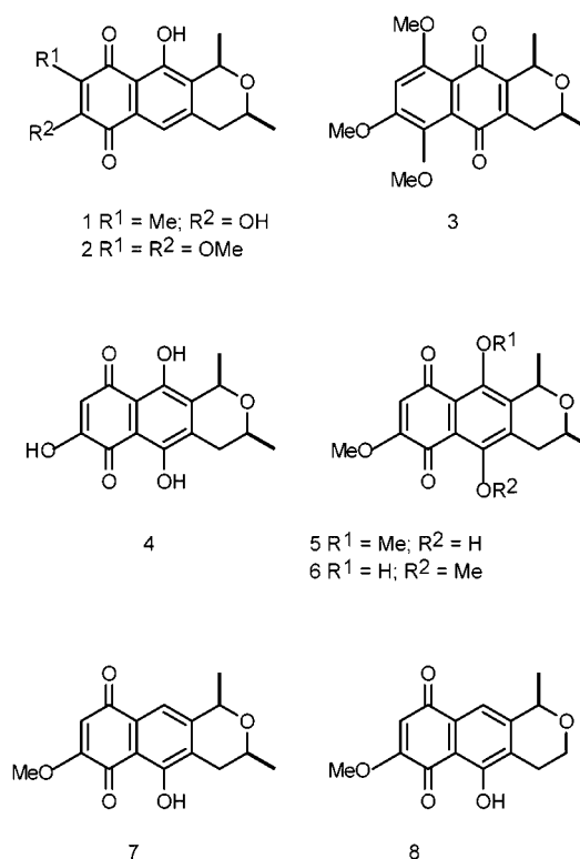
Figure 1. Examples of naphthophyranquinones
