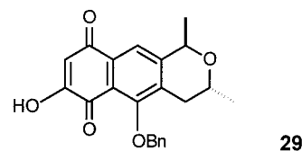
Figure 2. Hydrogenolysis product of 26
