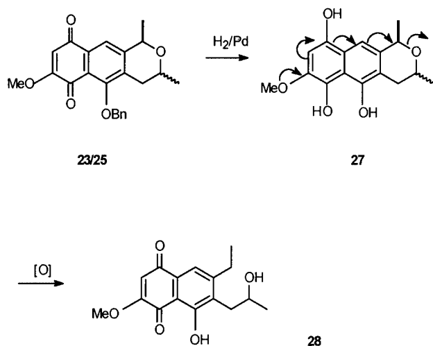
Scheme 3. Suggested mechanism for the formation of alcohol 28 derived from pyrans 23/25
